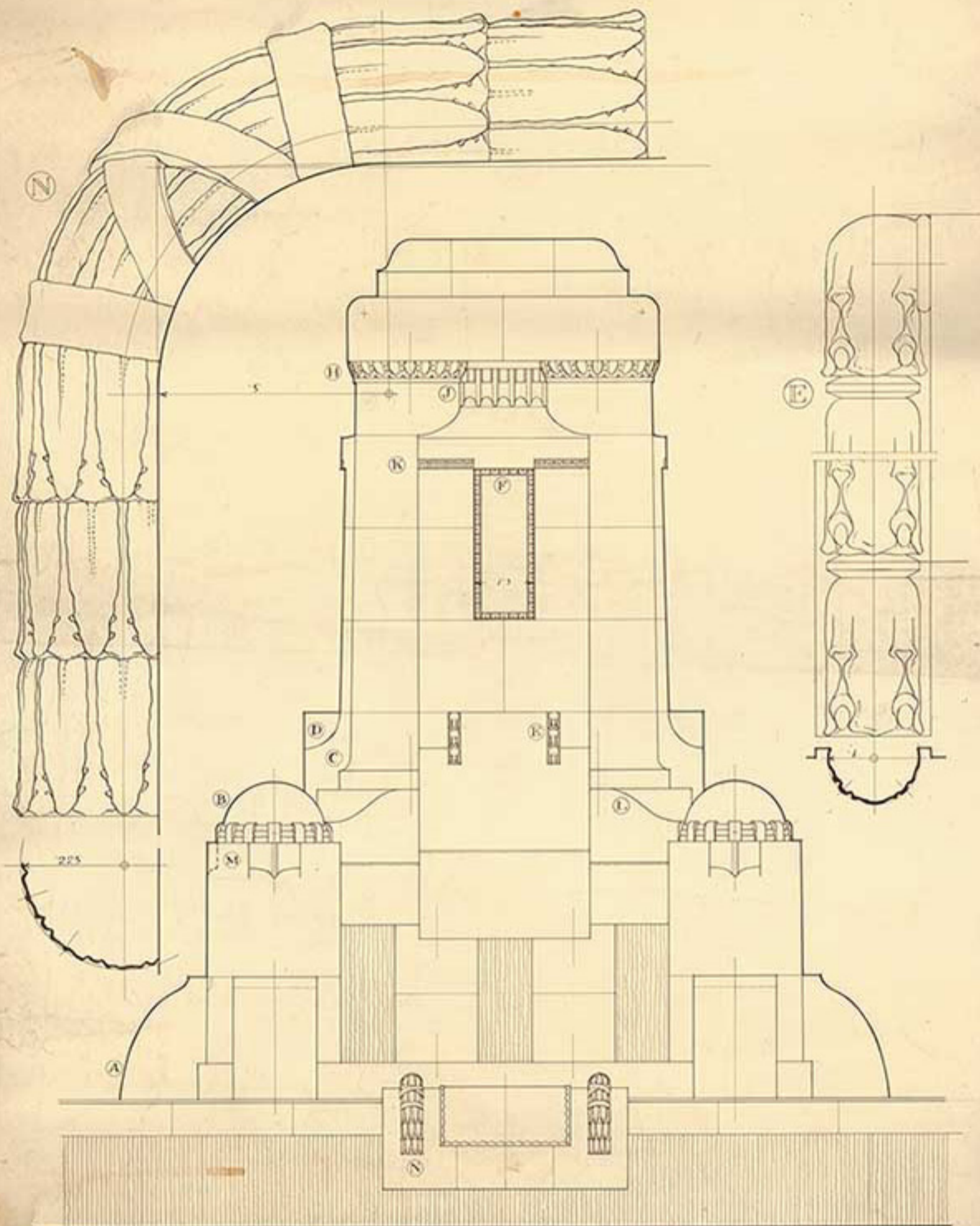
ELEVATION. SCALE 1:10
