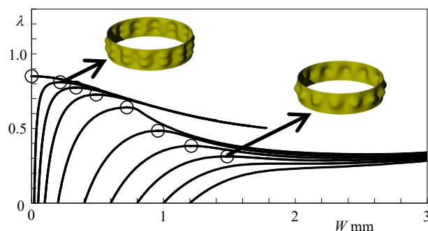
Fig.1 Load versus deflection curves for imperfect cylinders
