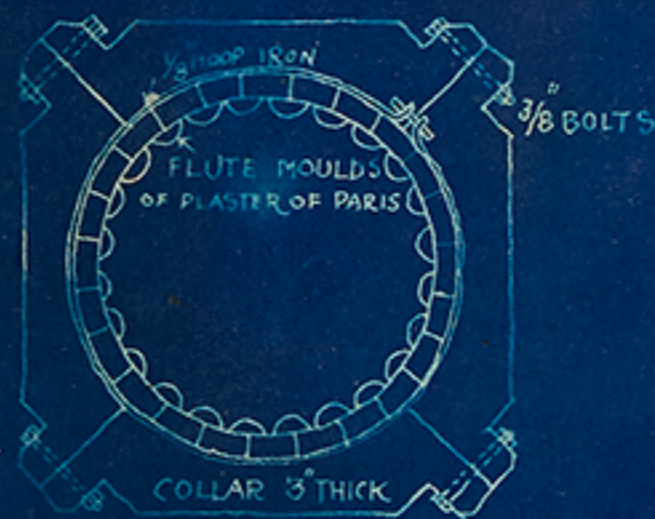
Fig. 248.—Form for Fluted Column
