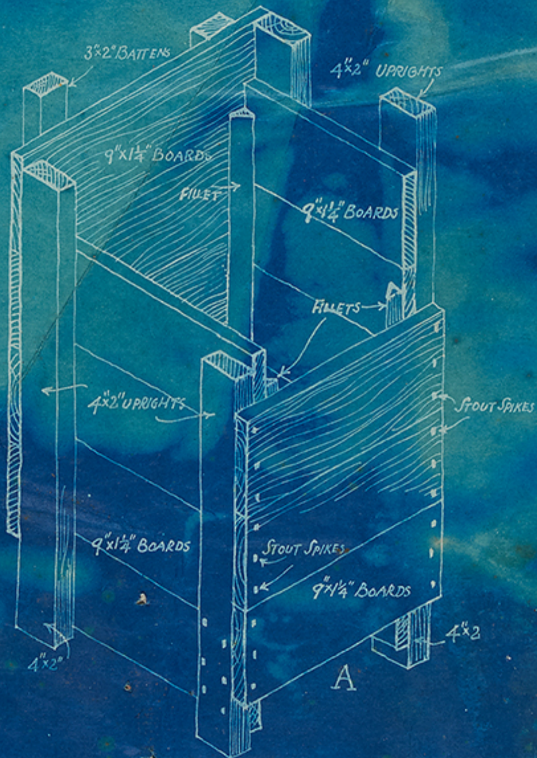
Fig. 221.—Typical Column Form with Spiked-on Front Boards
