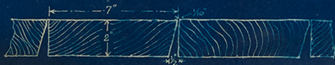
Fig. 227.—Boards with Splayed Edges to allow for Expansion
